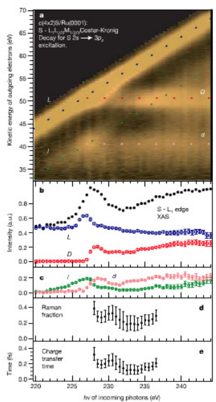
Figure 3 | Quantitative charge transfer analysis of sulphur L_{1,2,3}M_{4,5} Coster–Kronig autoionization spectra of c(4 \times 2)S/Ru(0001) as a function of photon energy. a , Experimental intensities as a function of incoming photon energy and kinetic energy of the outgoing electrons. Lighter colours correspond to higher autoionization intensity. Shown are Raman channels with linear dispersion for localized final states l ( 2p^{-1}3p^{-1}3p^1 ) at 170.7 eV binding energy and l ( 2p^{-1}3s^{-1}3p^1 ) at 181.7 eV binding energy, and charge transfer channels with delocalized final states d ( 2p^{-1}3p^{-1}deloc^1 ) at 50.8 eV kinetic energy and d ( 2p^{-1}3s^{-1}deloc^1 ) at 40.6 eV kinetic energy. b , Sum of spectral intensities representing the S-L 1 edge X-ray absorption spectrum. Also shown are separate intensities of the spectral channels ( l , d ) from curve fitting with Lorentzians of 3.3 eV FWHM. Error bars show the standard deviation of each fit. c , Separate intensities of the spectral channels ( l , d ) from curve fitting with Lorentzians of 3.3 eV FWHM. Error bars show the standard deviation of each fit. d , Raman fraction f = I(l+d) as a function of photon energy. Error bars are derived from the standard deviation of the fits (see c ). e , Charge transfer time obtained from the Raman fraction as \tau_{CT} = \tau f / (1-f) and the S 2s core-hole lifetime \tau = 0.5 fs. Error bars are derived from the standard deviation of the fits (see c ).
