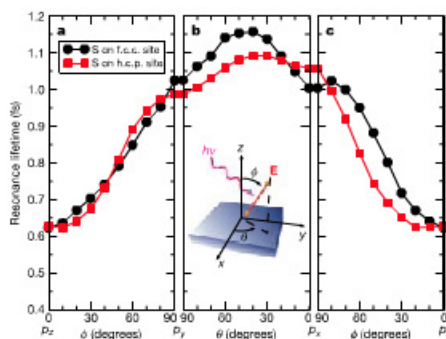
Figure 4 | Theoretical charge transfer time for S in f.c.c. and h.c.p. hollow sites computed as S 3p resonance lifetime. Theory predicts a strong dependence of the charge transfer time on the symmetry of the initial wave packet, which translates to a strong dependence on the light polarization. The coordinates x, y, z shown in the diagram in b correspond to the crystallographic directions [100], [010], [001]. The circles and squares correspond respectively to sulphur atoms in f.c.c. and h.c.p. sites of the surface. a , Resonance lifetime as a function of the angle \phi of the electric field vector with respect to the surface normal in the y - z plane. Polarization of the synchrotron light along the z axis ( \phi = 0 , the experimental geometry) produces an initial excited state with p_z symmetry. b , Resonance lifetime as a function of the angle \theta of the electric field vector with respect to the x axis in the x - y plane. In this geometry, p_x and p_y symmetries and combinations of them would be obtained with in-plane polarization. c , Resonance lifetime as a function of the angle \phi of the electric field vector with respect to the surface normal in the x - z plane.
