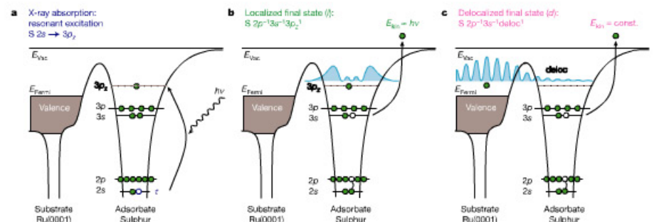
Figure 1 Core-hole clock spectroscopy—schematic overview. a , Initially, a core electron is promoted by resonant excitation from the S 2s level into a bound resonance localized at an adsorbed sulphur atom (S 2s -1 3p z ) on ruthenium c(4 × 2)S/Ru(0001) with a core-hole lifetime \tau = 0.5 fs. In the autoionization decay processes, Coster-Kronig decay of the S 2s core hole takes place in the presence of this electron, the so-called 'spectator' electron,
